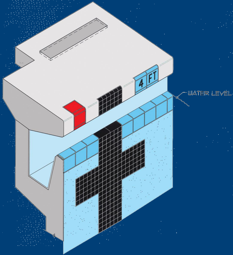
Cantilever Gutter
